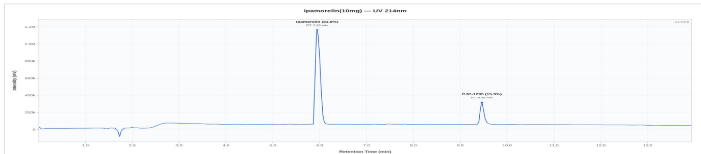
CJC-1295 Without DAC 5mg+IPA 10mg - CJC-2026-001: UV Chromatogram
